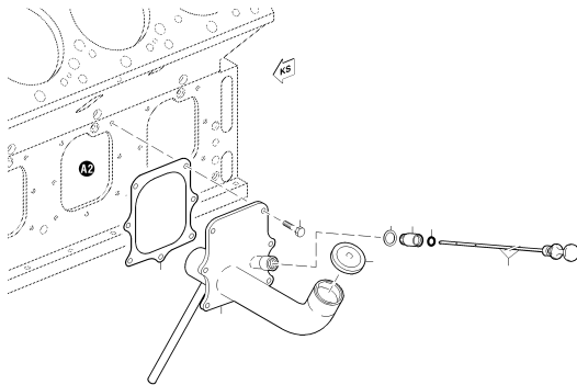
OIL FILLER NECK WITH OIL DIPSTICK XS526010.00009
